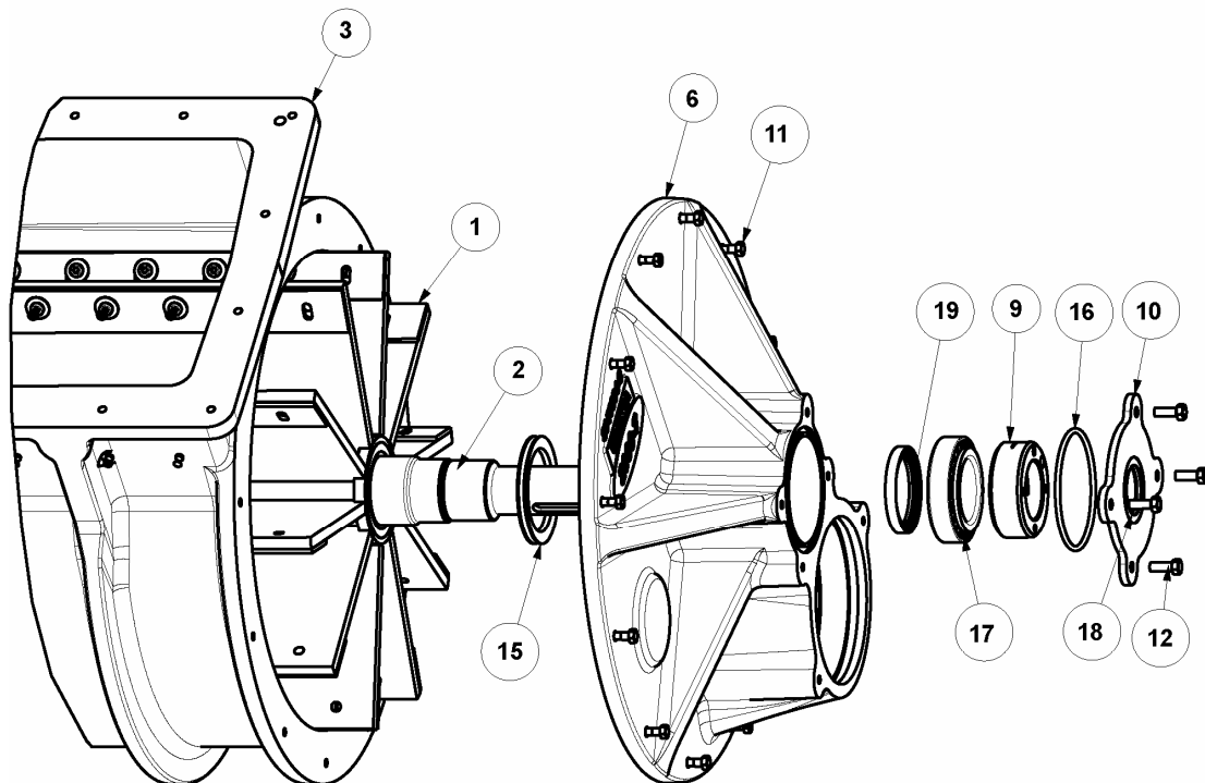
Fig. 1.4 2018 Exploded View
